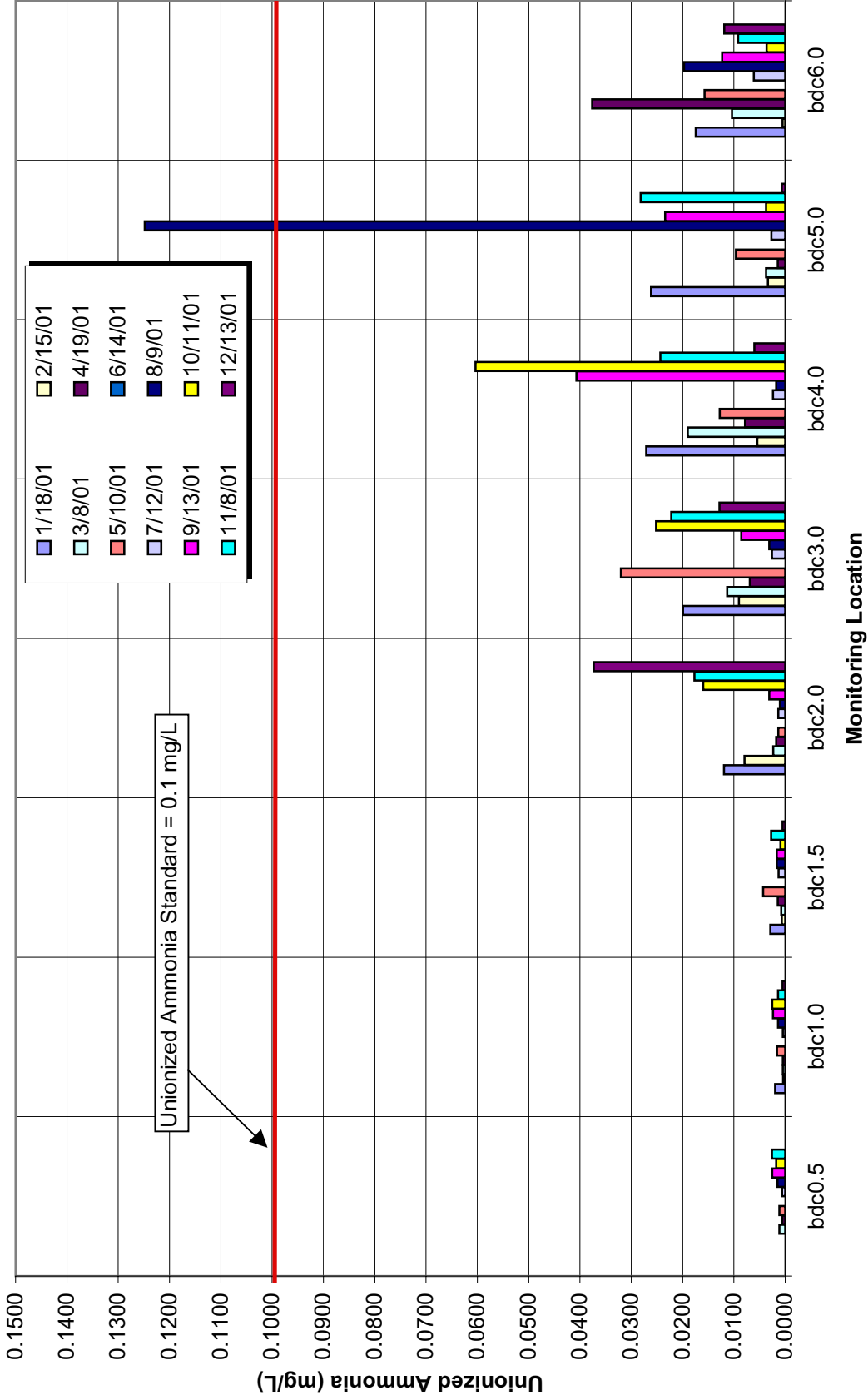
Figure 7 Monthly Unionized Ammonia Concentrations for Big Dry Creek 2001
